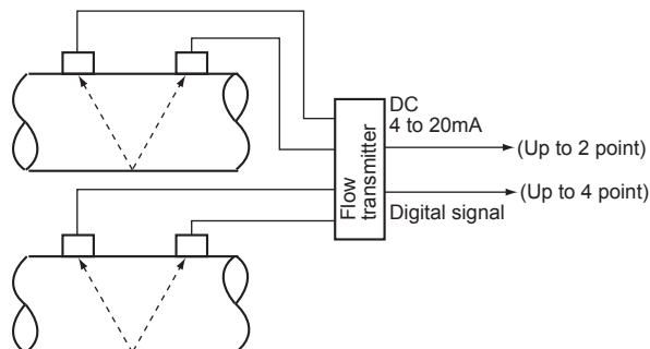
(5) 2-pipe system (V method)
